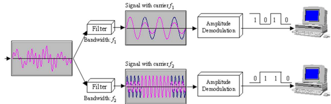
FDM demultiplexing process
