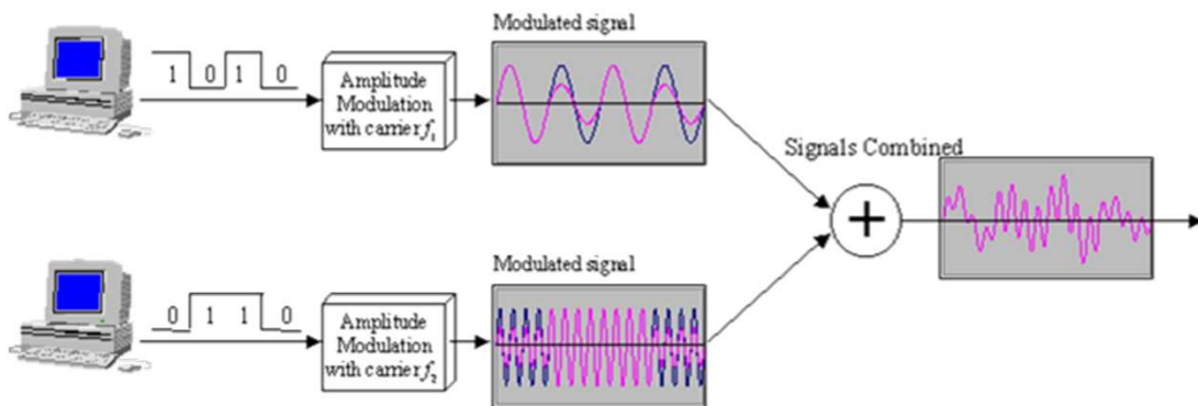
FDM multiplexing process
